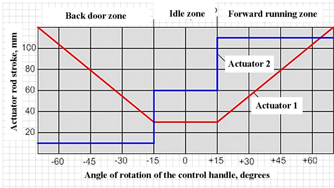
Figure 10. Characteristics of the actuators of the Mini-Marex DAU system.
