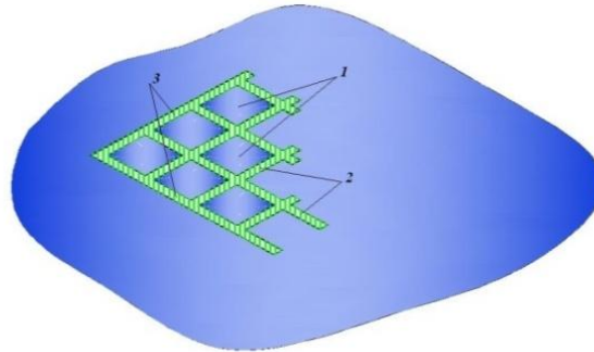
Figure 8. Scheme of the developed area after the construction of dividing artificial massifs: 1 - extraction units; 2 and 3 - respectively, dividing and delineating artificial massifs prospects and for a radical solution to environmental problems in the development of ore deposits.
