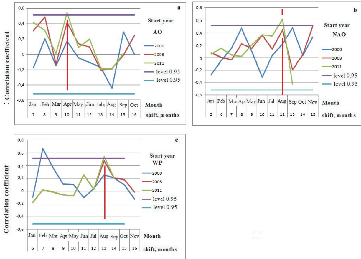
Figure 3. Dependences of the correlation coefficient of the 15-year segments of the AO, NAO, and WP time series, as well as the segments of the MAT G series leading them in time, on the time shift between them, for the months to which the MAT G series correspond
