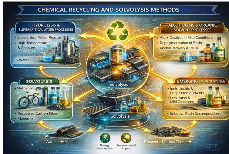
Figure 2. Common chemical recycling and solvolysis methods.
