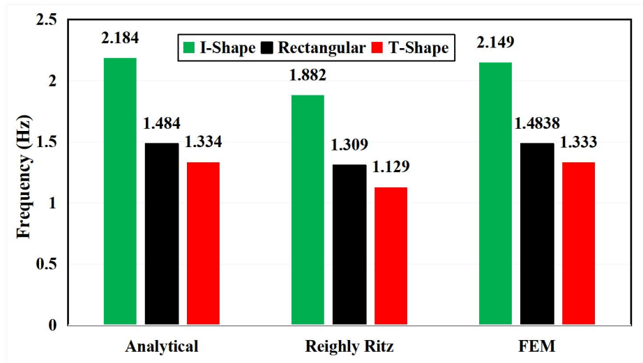
Figure 6. Frequency comparison among different cross-sectional geometries.
