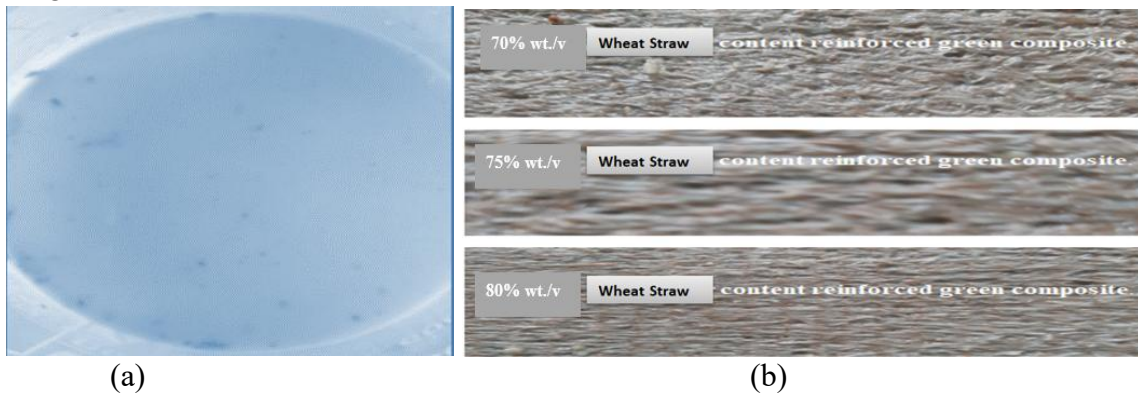
Figure 2. Lab made bio resin and green composite fabrication: (a) Lab made bio resin from mixed Abyssinica glue and Ficus vasta (Warka) gum (b) Biodegradable composite.
