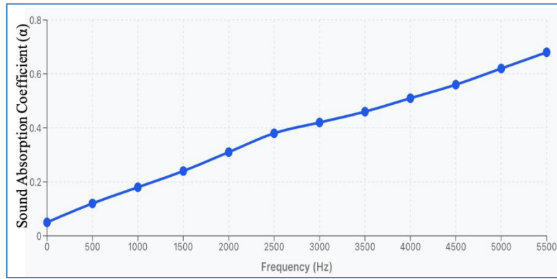
Figure.4. Sound absorption coefficients (6.0 mm thickness) wheat straw fibrous material reinforced green composite.
