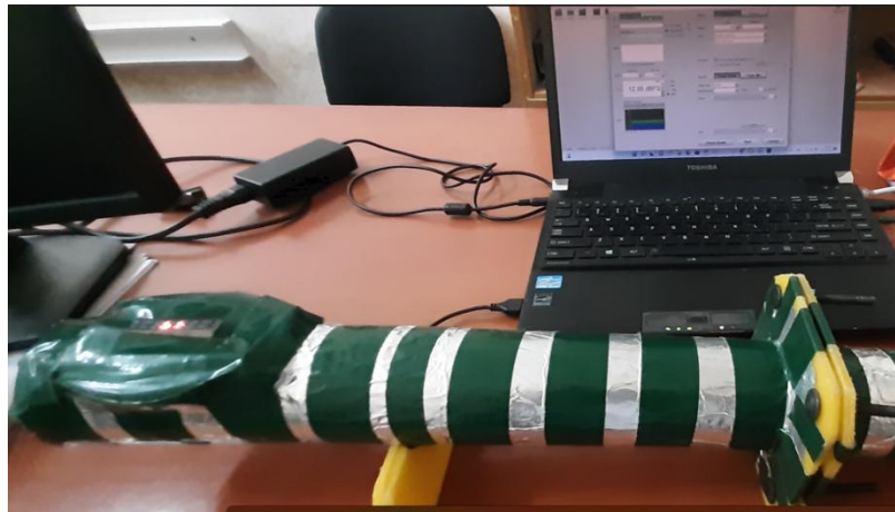
Figure 3. Impedance tube; Double-microphones standing wave tube.
