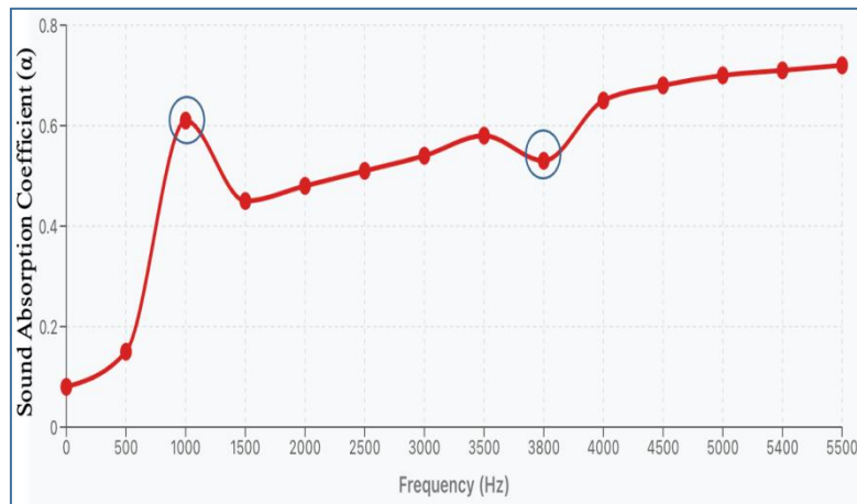
Figure. 5. Sound absorption coefficient (8.0 mm thickness) wheat straw fibrous material reinforced green composite.
