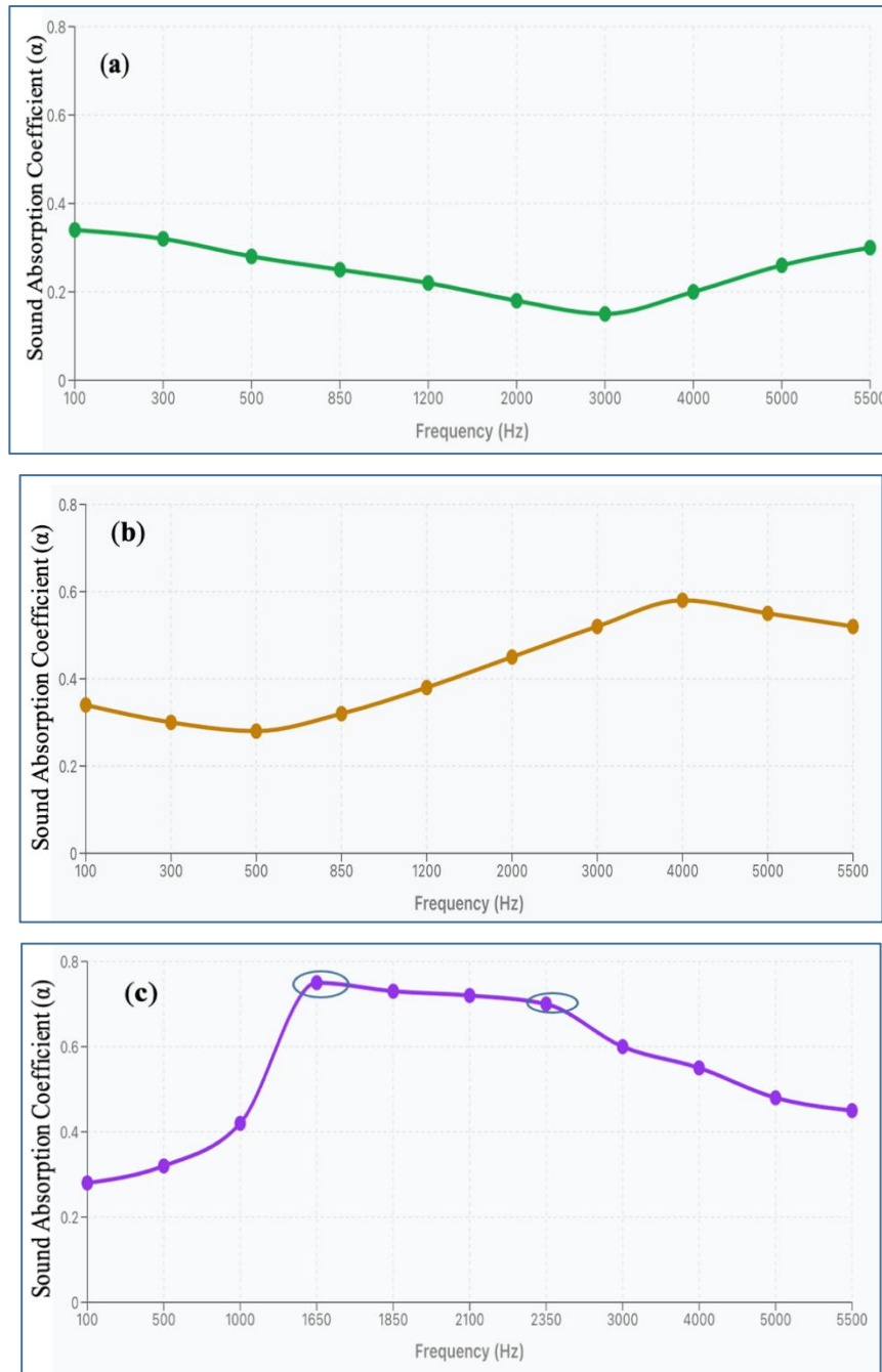
Figure 6. Sound absorption coefficient ( \alpha ): (a) 30 % wt./v Wheat straw fibrous material content, (b) 25 % wt./v Wheat straw fibrous material content, (c) 20 % wt./v Wheat straw fibrous material content reinforced green composite.
