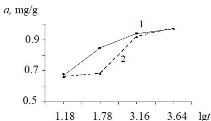
Figure 2. Dependence of the sorption capacity ( a ) of coal mining waste rocks when absorbing the MB dye on time ( t ): 1 for unburnt rock of the Khmel'nitskaya mine; 2 for unburnt rock of the Sverdlov mine.
