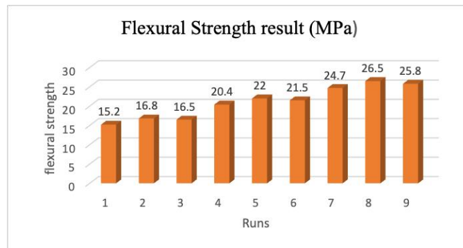
Figure 4. Flexural strength test result.
