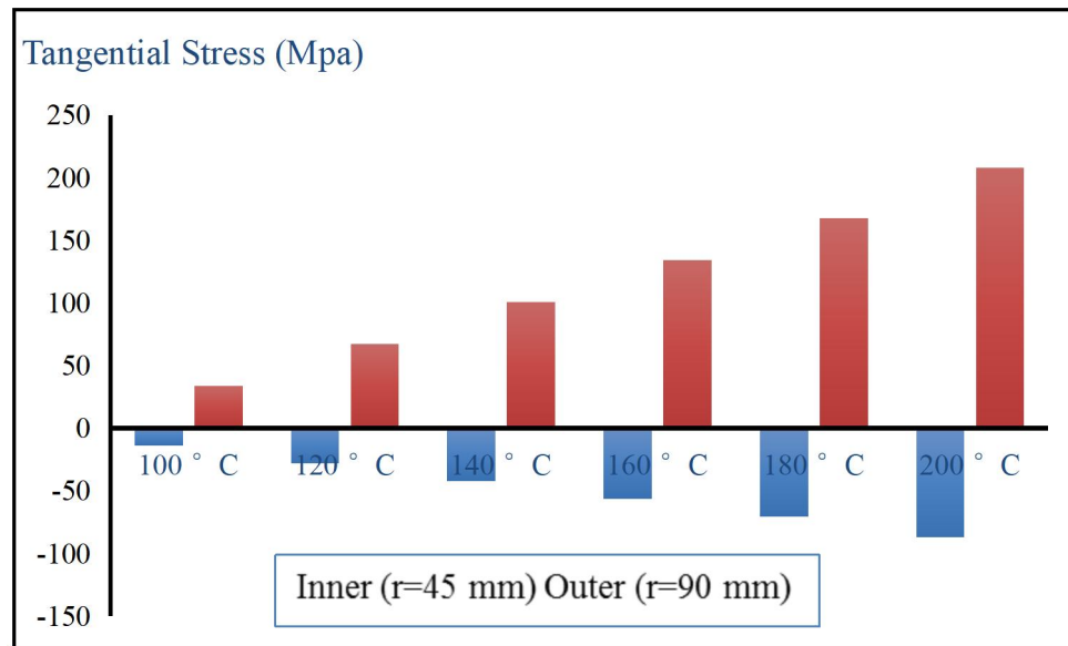
Figure 5. Tangential stresses occurring at the inner and outer regions of the silicon nitride ( \text{Si}_3\text{N}_4 ) disk.
